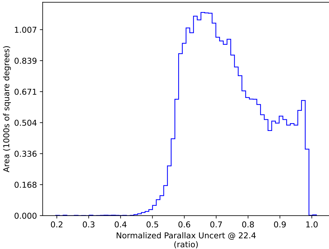
ddf_acor_sf15_lsf40_lsr20_v3.4_10yrs : Normalized Parallax Uncert @ 22.4
