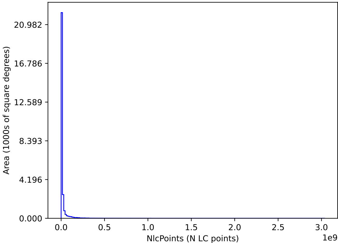
ddf_acor_sf15_lsf40_lsr20_v3.4_10yrs : NlcPoints
