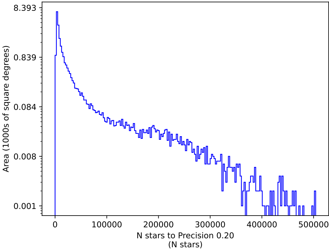
ddf_acor_sf15_lsf40_lsr20_v3.4_10yrs u: N stars to Precision 0.20
