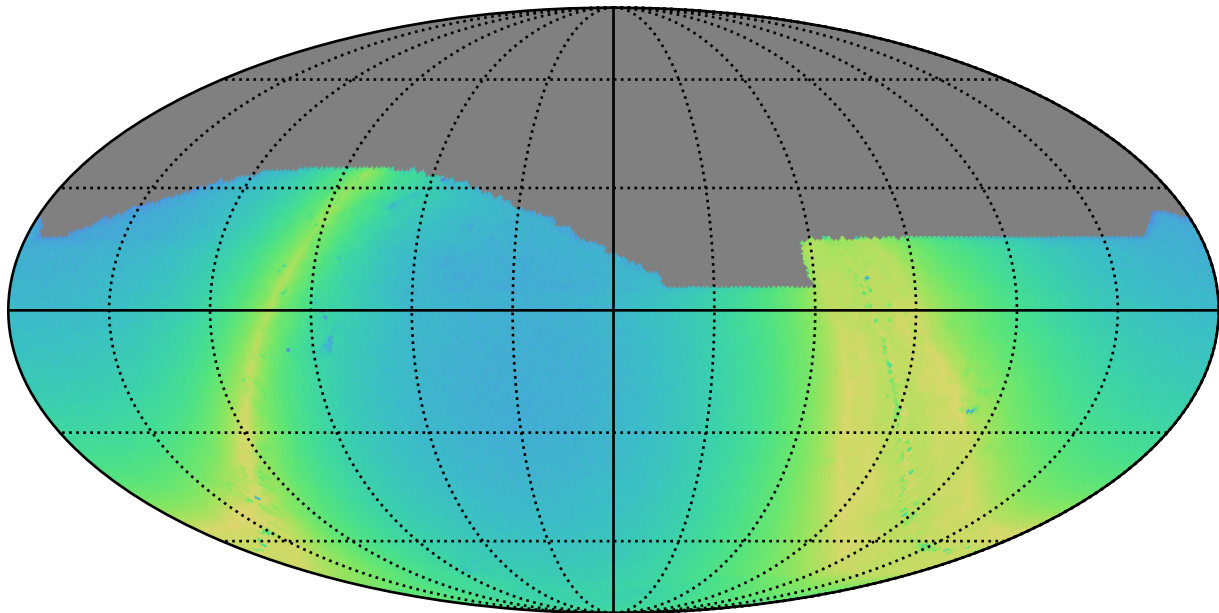
ddf_acor_sf15_lsf40_lsr20_v3.4_10yrs i: N stars to Precision 0.20
