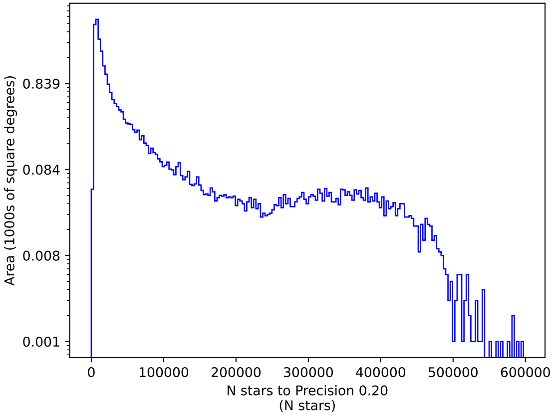
ddf_acor_sf15_lsf40_lsr20_v3.4_10yrs g: N stars to Precision 0.20
