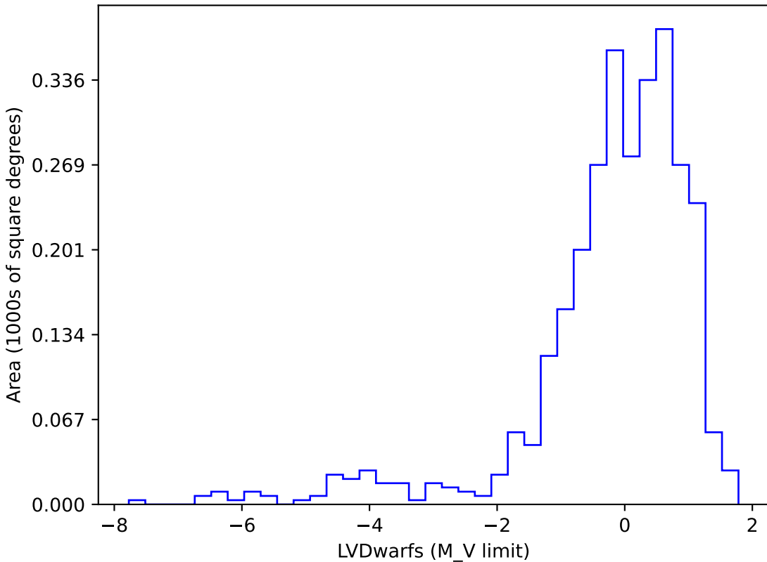
ddf_acor_sf15_lsf40_lsr20_v3.4_10yrs gi SCP: LVDwarfs
