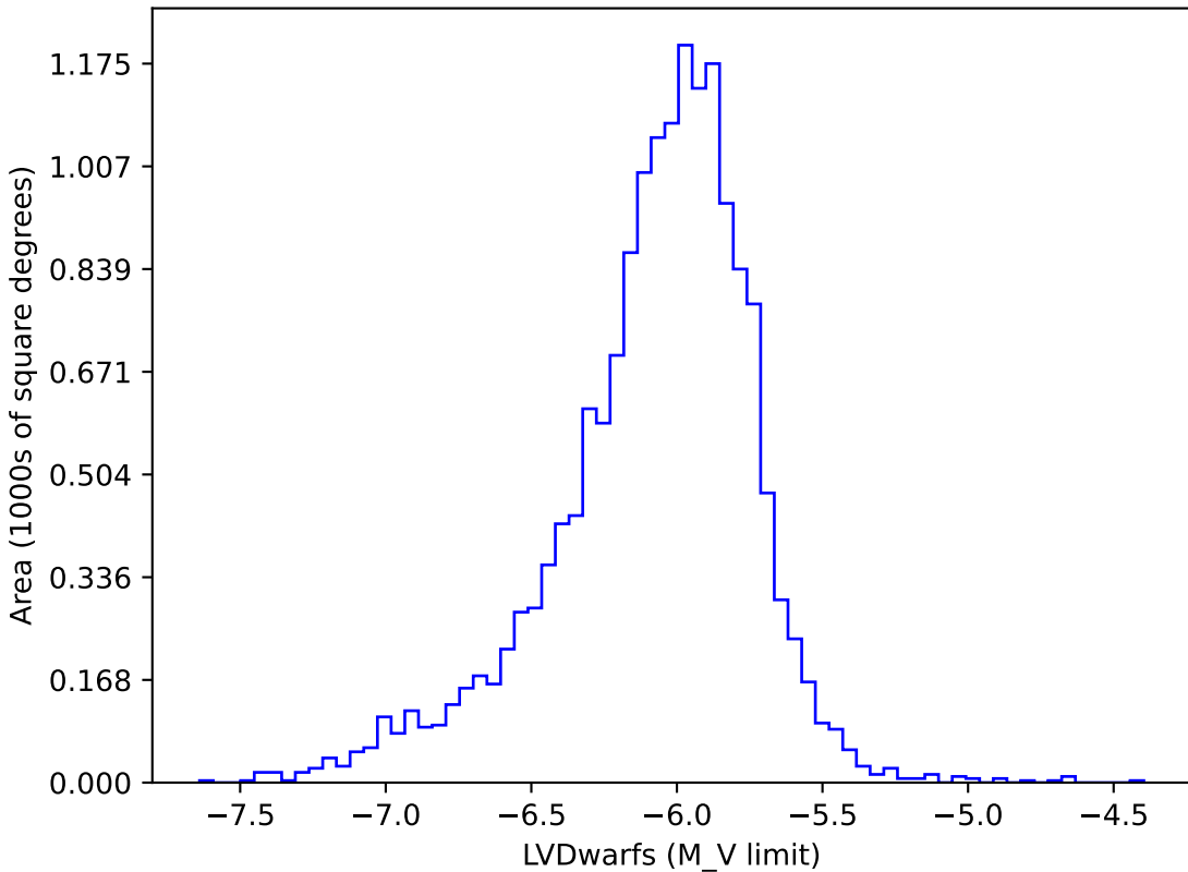
ddf_acor_sf15_lsf40_lsr20_v3.4_10yrs gi: LVDwarfs
