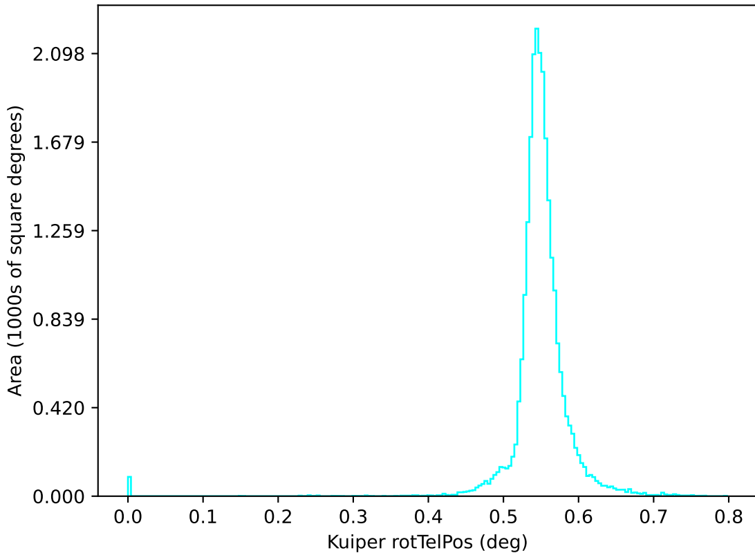
ddf_acor_sf15_ls40_lsr20_v3.4_10yrs u: Kuiper rotTelPos
