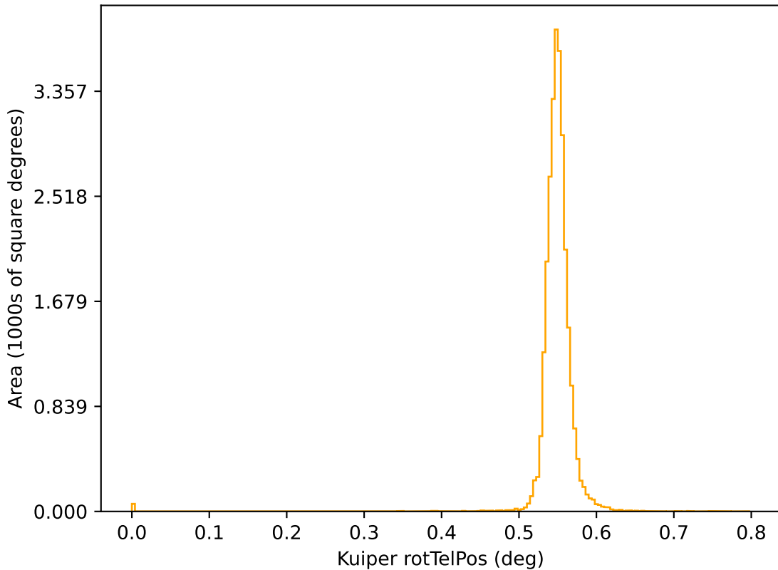
ddf_acor_sf15_lsf40_lsr20_v3.4_10yrs r: Kuiper rotTelPos
