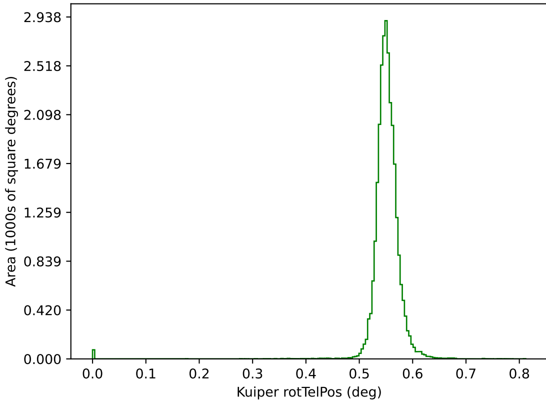
ddf_acor_sf15_lsf40_lsr20_v3.4_10yrs g: Kuiper rotTelPos
