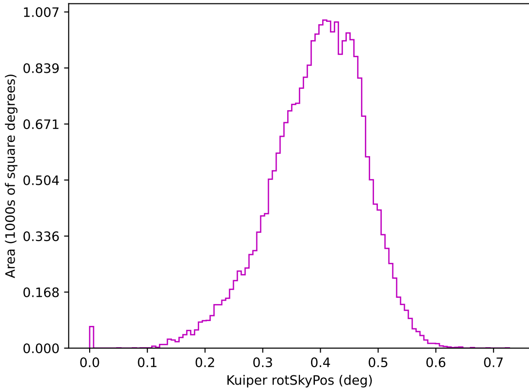
ddf_acor_sf15_lsf40_lsr20_v3.4_10yrs z: Kuiper rotSkyPos
