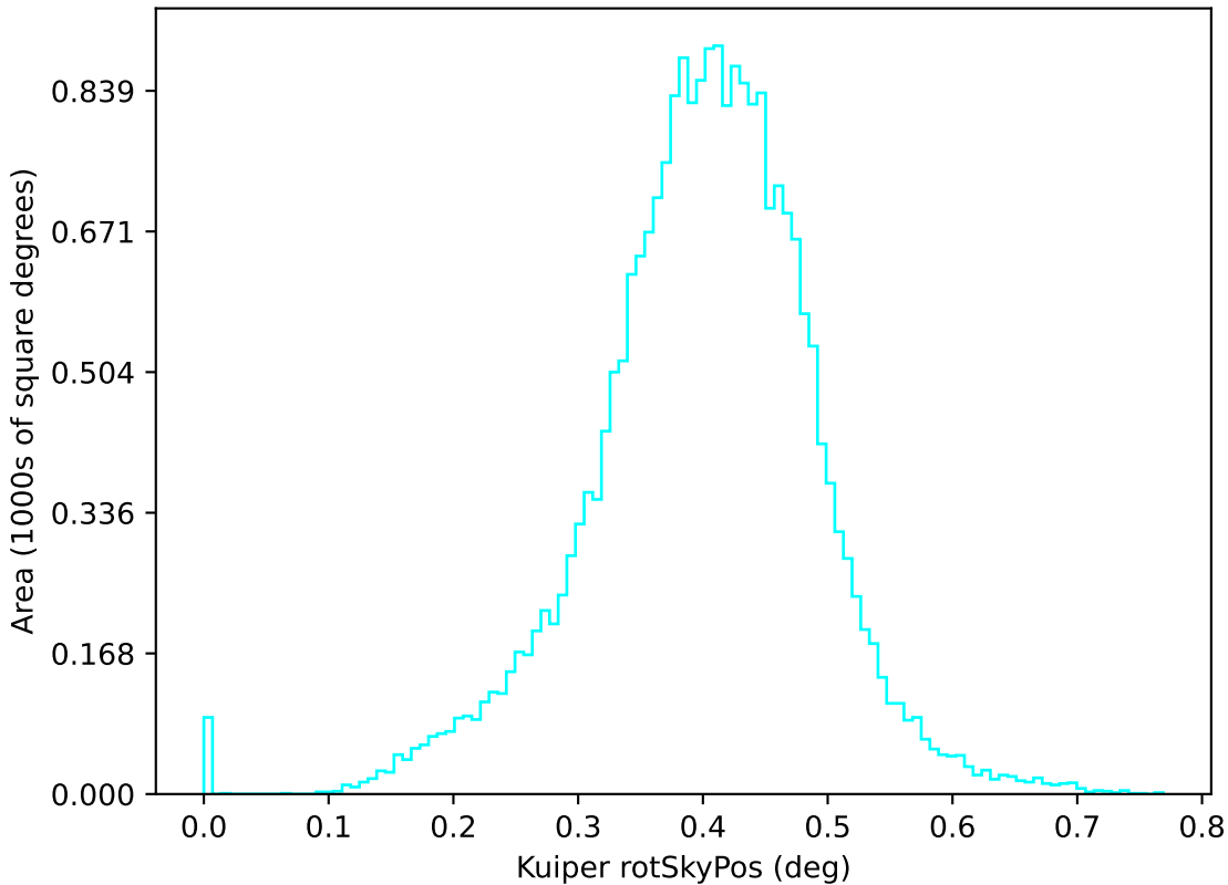
ddf_acor_sf15_lsf40_lsr20_v3.4_10yrs u: Kuiper rotSkyPos
