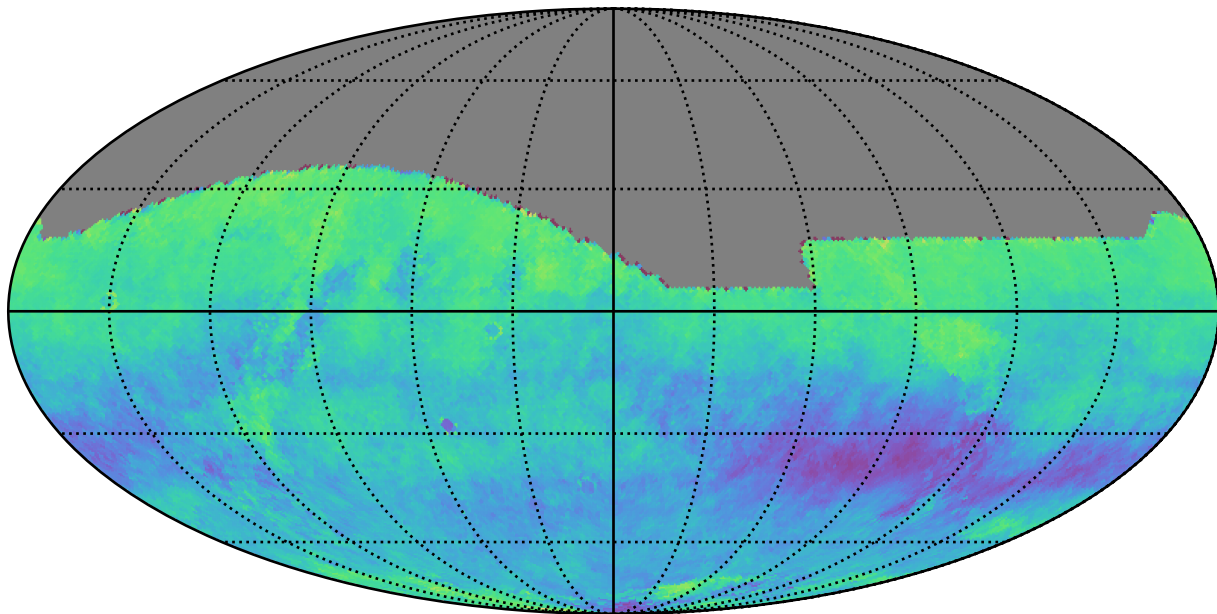
ddf_acor_sf15_lsf40_lsr20_v3.4_10yrs r: Kuiper rotSkyPos
