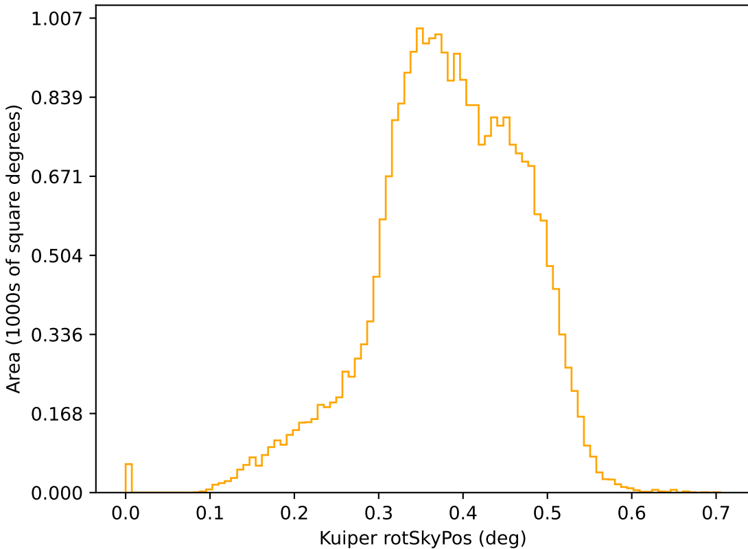
ddf_acor_sf15_lsf40_lsr20_v3.4_10yrs r: Kuiper rotSkyPos
