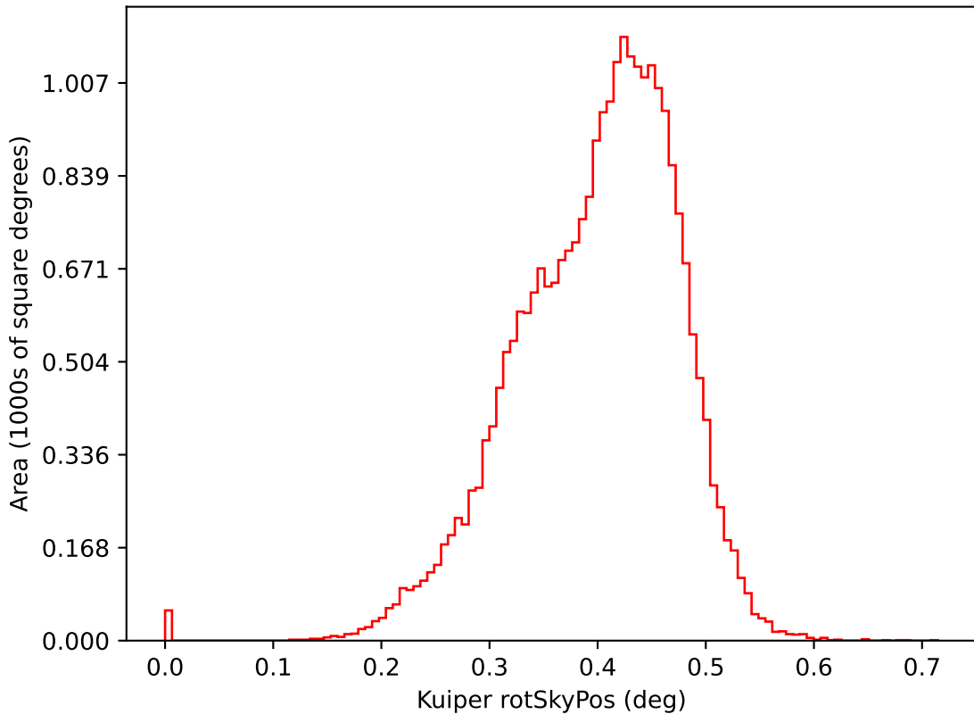
ddf_acor_sf15_lsf40_lsr20_v3.4_10yrs i: Kuiper rotSkyPos
