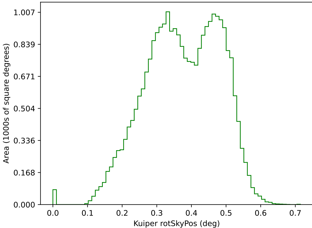
ddf_acor_sf15_lsf40_lsr20_v3.4_10yrs g: Kuiper rotSkyPos
