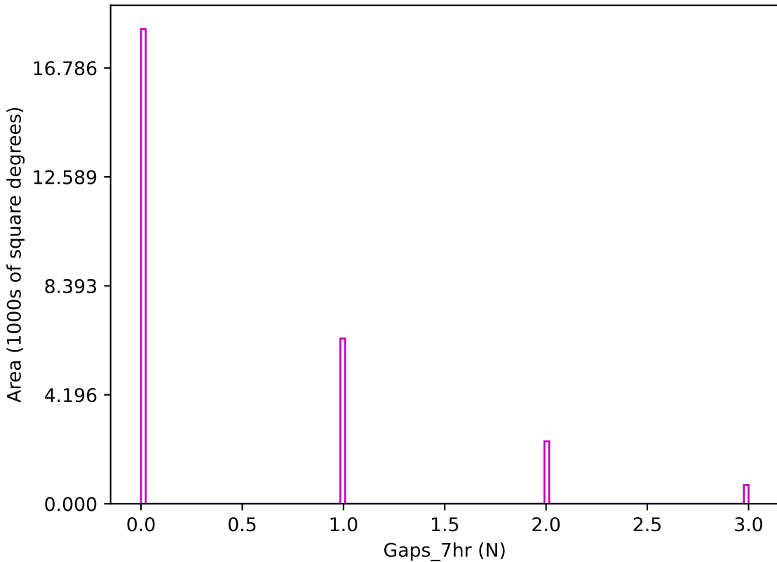
ddf_acor_sf15_ls40_lsr20_v3.4_10yrs z band: Gaps_7hr
