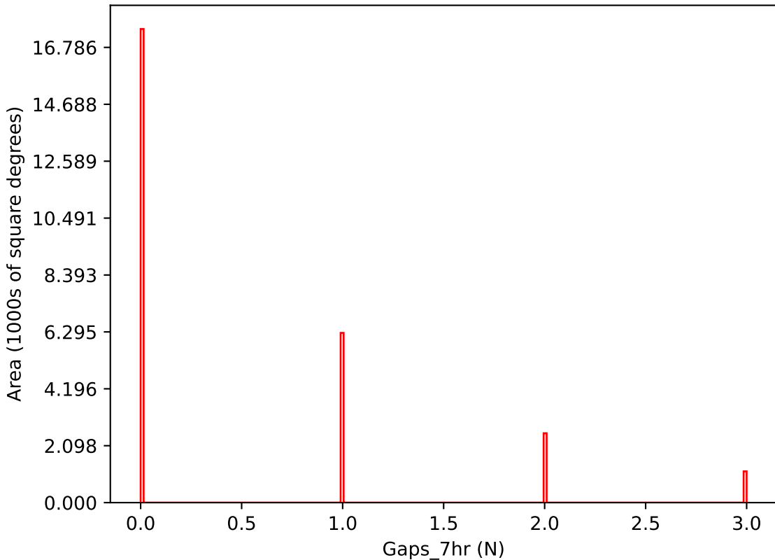
ddf_acor_sf15_lsf40_lsr20_v3.4_10yrs i band: Gaps_7hr
