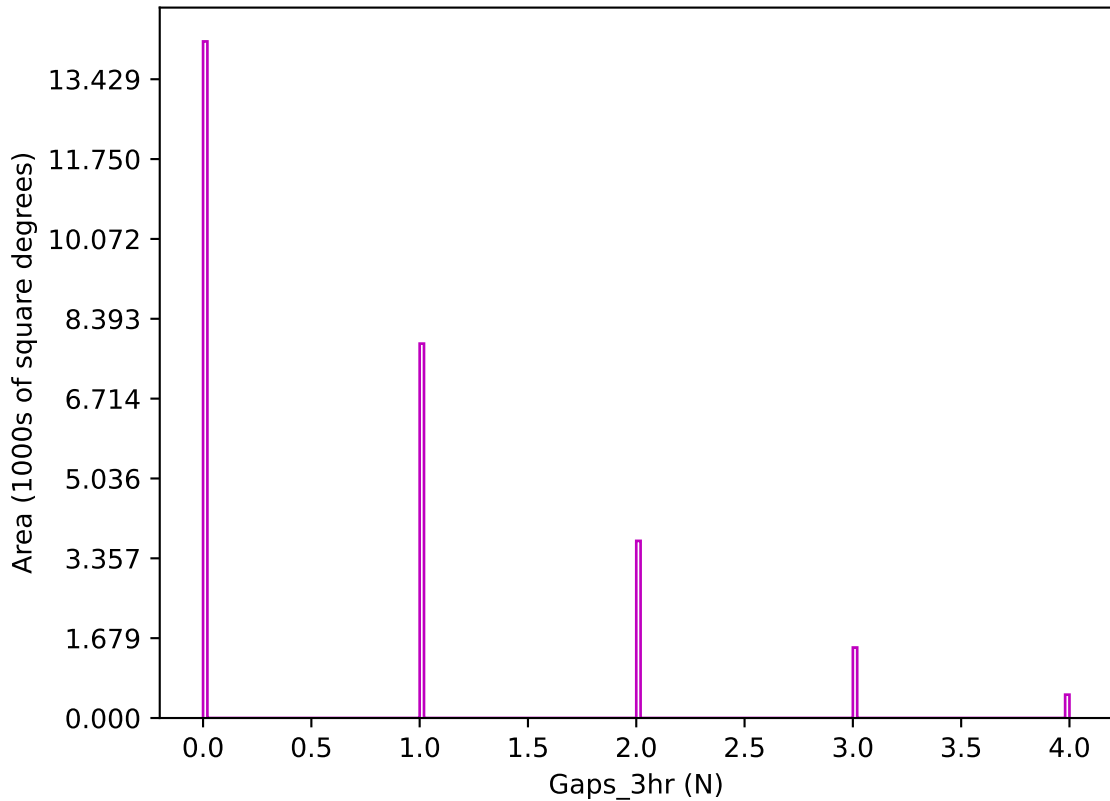
ddf_acor_sf15_ls40_lsr20_v3.4_10yrs z band: Gaps_3hr
