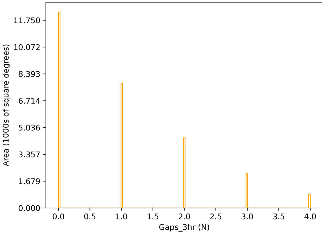
ddf_acor_sf15_lsf40_lsr20_v3.4_10yrs r band: Gaps_3hr
