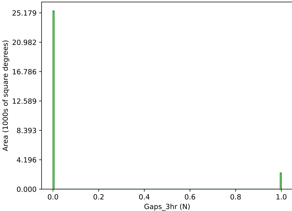
ddf_acor_sf15_lsf40_lsr20_v3.4_10yrs g band: Gaps_3hr
