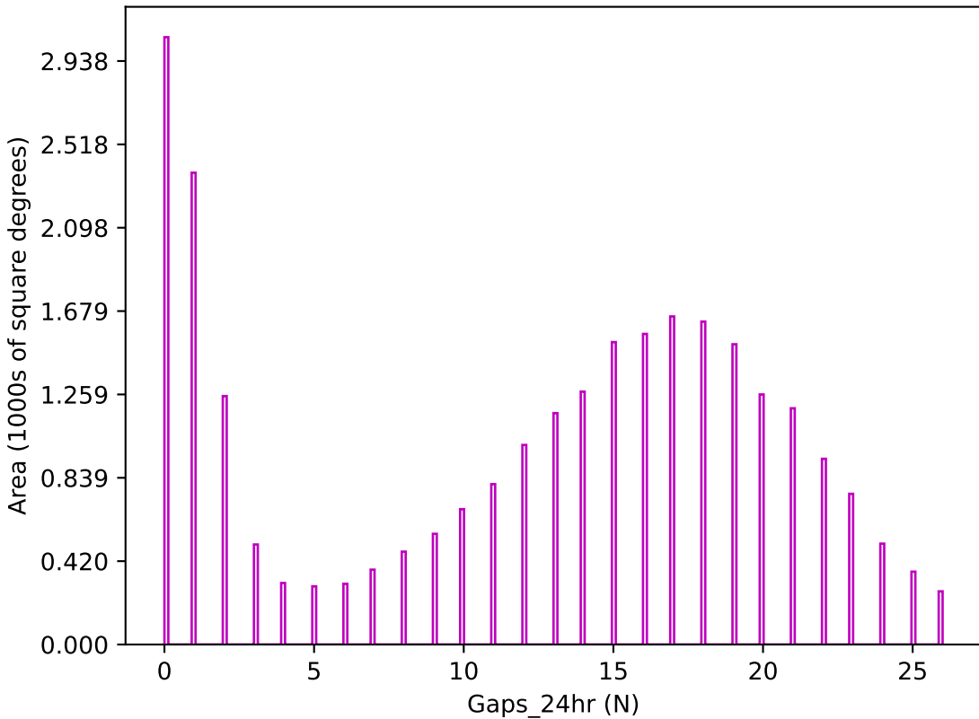
ddf_acor_sf15_ls40_lsr20_v3.4_10yrs z band: Gaps_24hr
