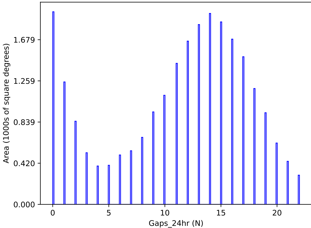
ddf_acor_sf15_lsf40_lsr20_v3.4_10yrs y band: Gaps_24hr
