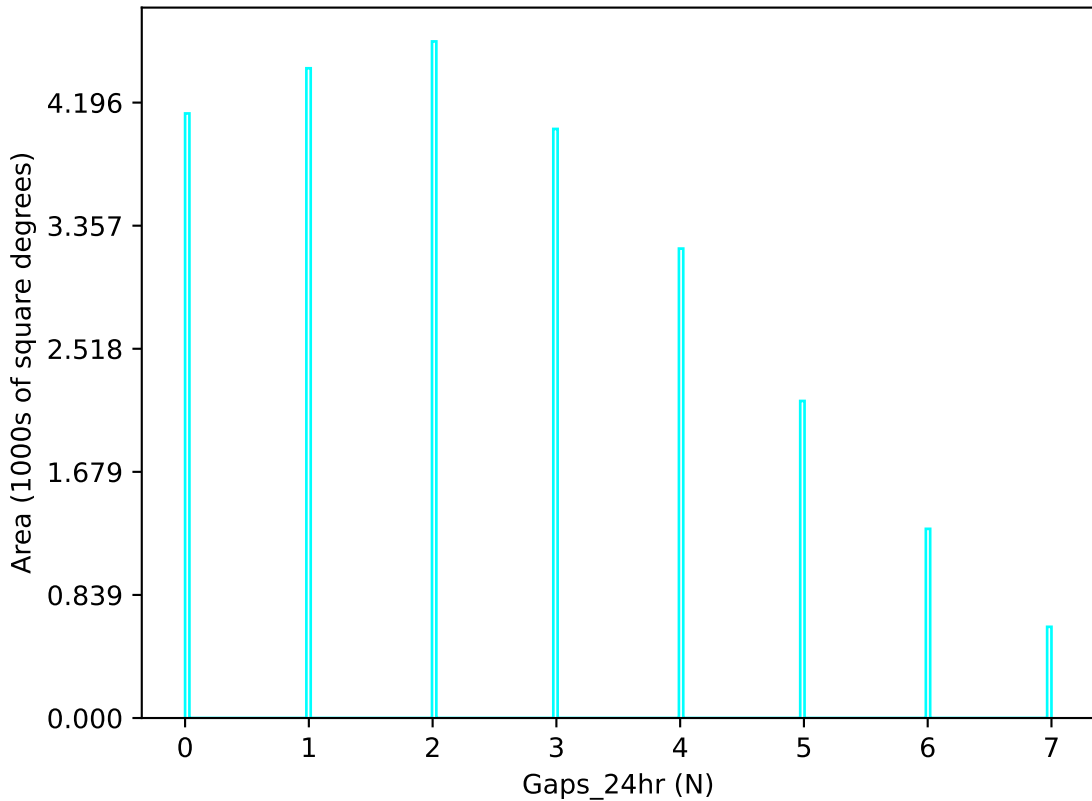
ddf_acor_sf15_lsf40_lsr20_v3.4_10yrs u band: Gaps_24hr
