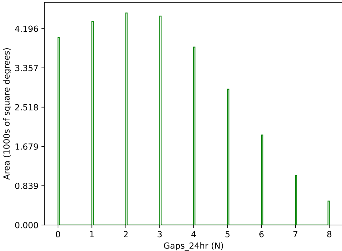
ddf_acor_sf15_lsf40_lsr20_v3.4_10yrs g band: Gaps_24hr
