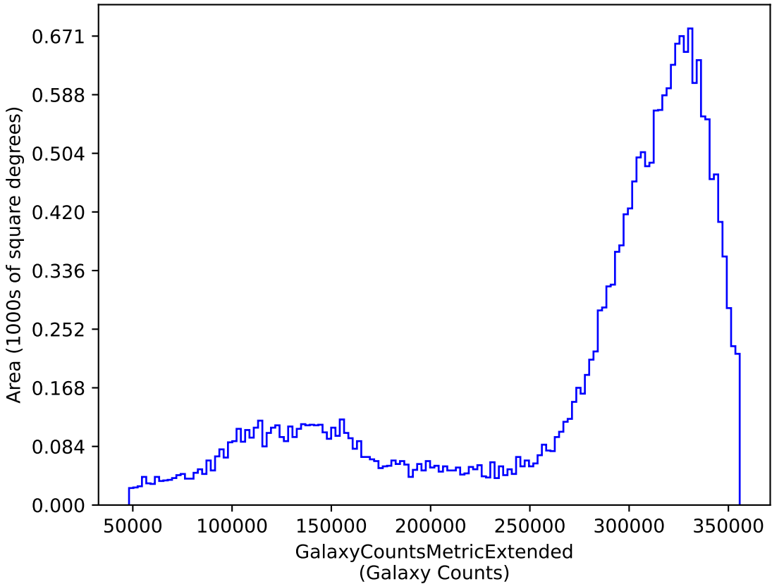
ddf_acor_sf15_lsf40_lsr20_v3.4_10yrs y: GalaxyCountsMetricExtended
