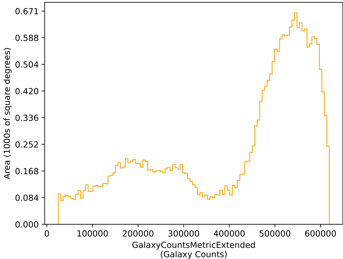
ddf_acor_sf15_lsf40_lsr20_v3.4_10yrs r: GalaxyCountsMetricExtended
