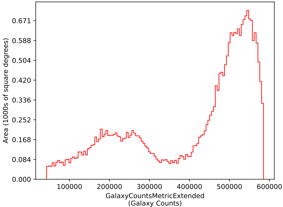
ddf_acor_sf15_ls40_lsr20_v3.4_10yrs i: GalaxyCountsMetricExtended
