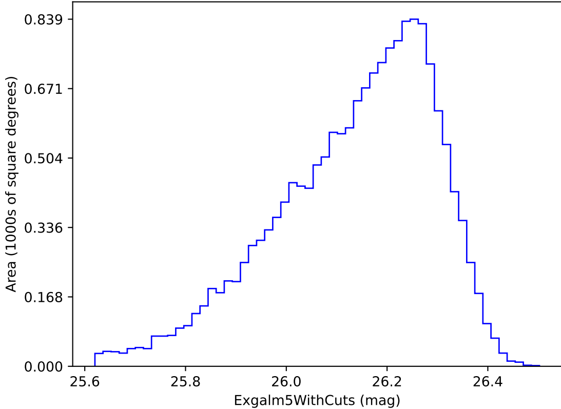
ddf_acor_sf15_lsf40_lsr20_v3.4_10yrs i band non-DD year 6: ExgalM5WithCuts
