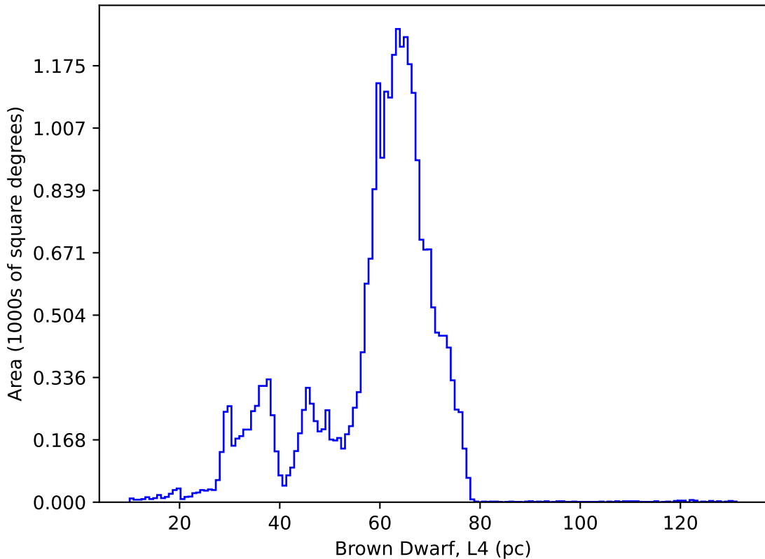
ddf_acor_sf15_lsf40_lsr20_v3.4_10yrs : Brown Dwarf, L4
