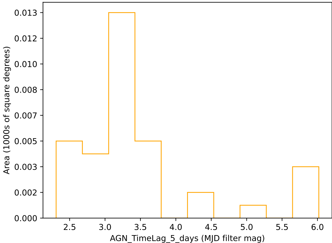
ddf_acor_sf15_lsf40_lsr20_v3.4_10yrs r band: AGN_TimeLag_5_days
