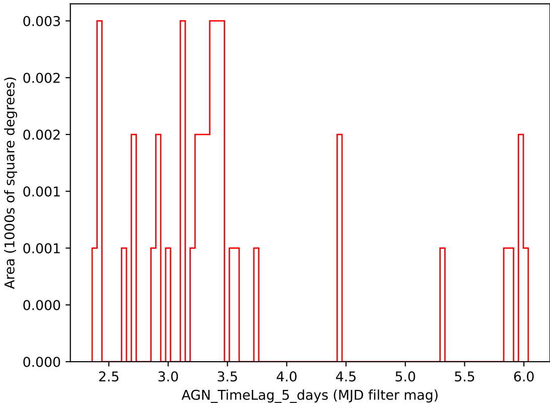
ddf_acor_sf15_lsf40_lsr20_v3.4_10yrs i band: AGN_TimeLag_5_days
