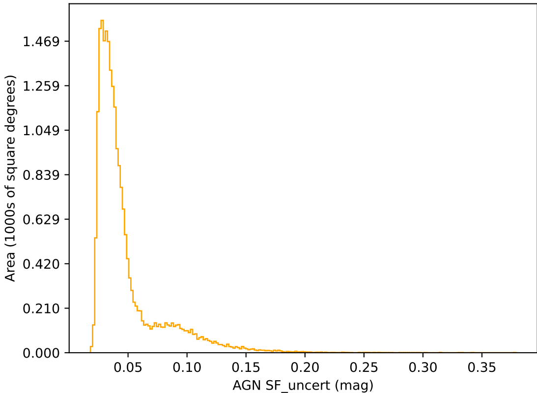
ddf_acor_sf15_lsf40_lsr20_v3.4_10yrs r band: AGN SF_uncert
