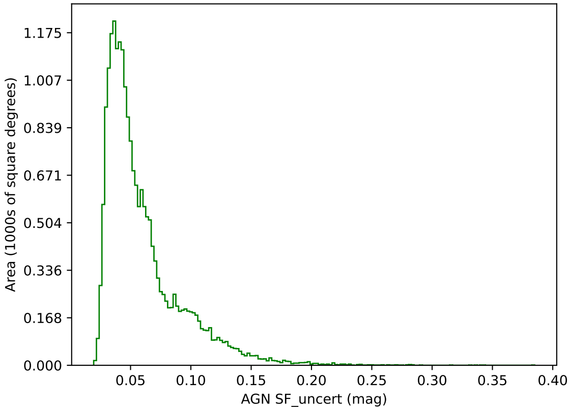
ddf_acor_sf15_lsf40_lsr20_v3.4_10yrs g band: AGN SF_uncert
