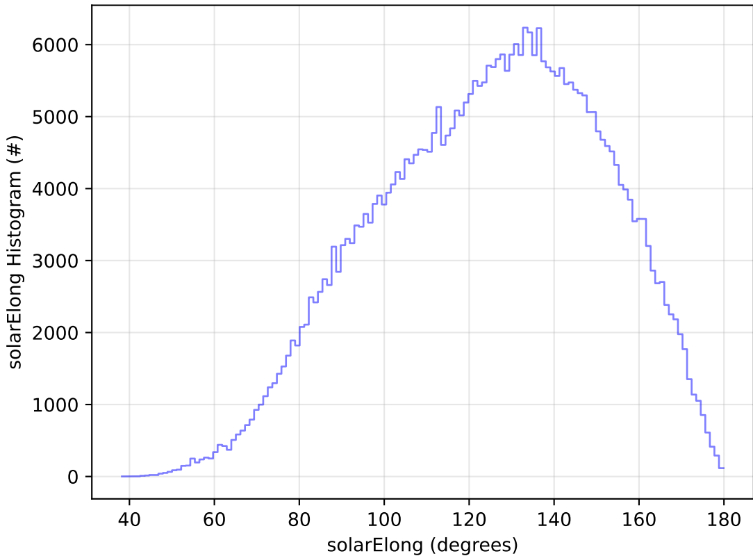
ddf_acor_sf15_lsf40_lsr20_v3.4_10yrs WFD y band: solarElong Histogram
