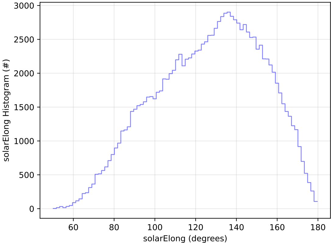
ddf_acor_sf15_lsf40_lsr20_v3.4_10yrs WFD u band: solarElong Histogram
