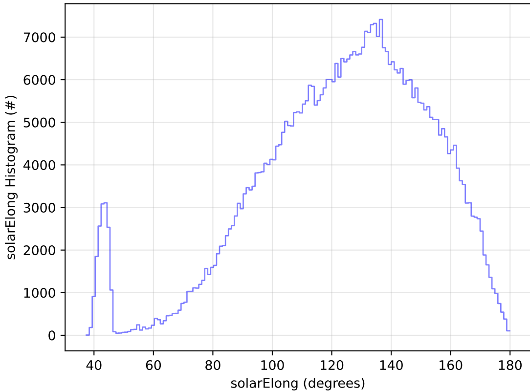
ddf_acor_sf15_ls40_lsr20_v3.4_10yrs WFD r band: solarElong Histogram
