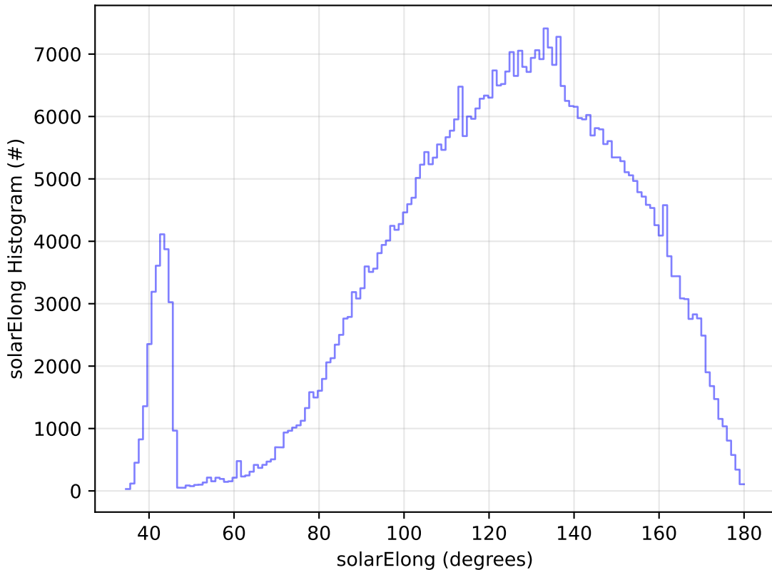
ddf_acor_sf15_lsf40_lsr20_v3.4_10yrs WFD i band: solarElong Histogram
