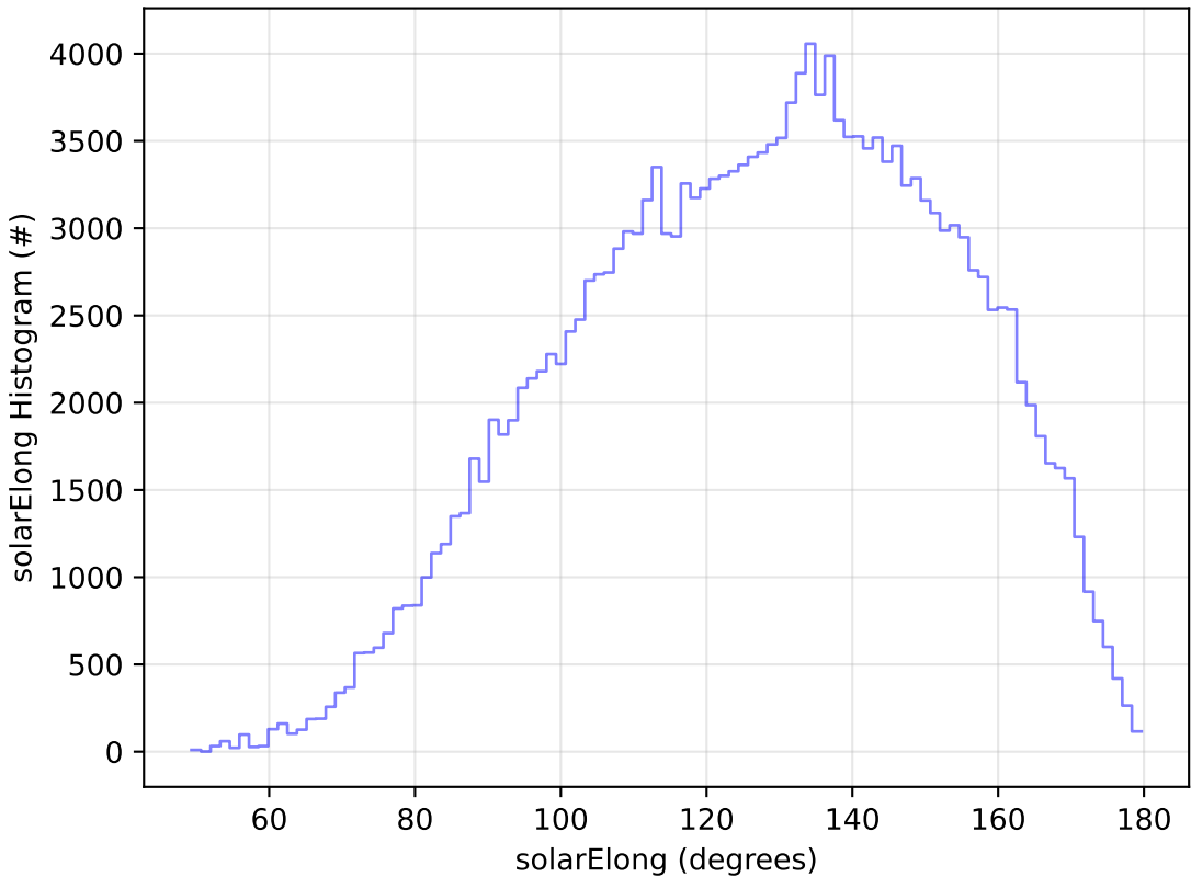
ddf_acor_sf15_lsf40_lsr20_v3.4_10yrs WFD g band: solarElong Histogram
