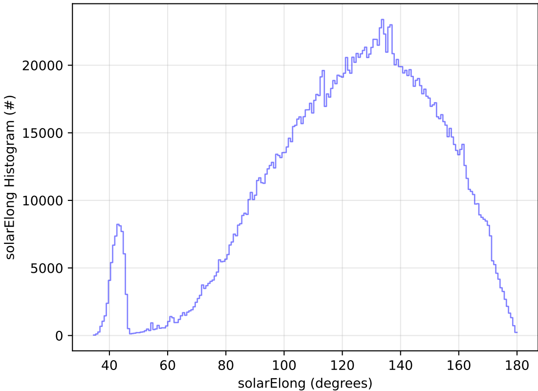
ddf_acor_sf15_lsf40_lsr20_v3.4_10yrs WFD all bands: solarElong Histogram
