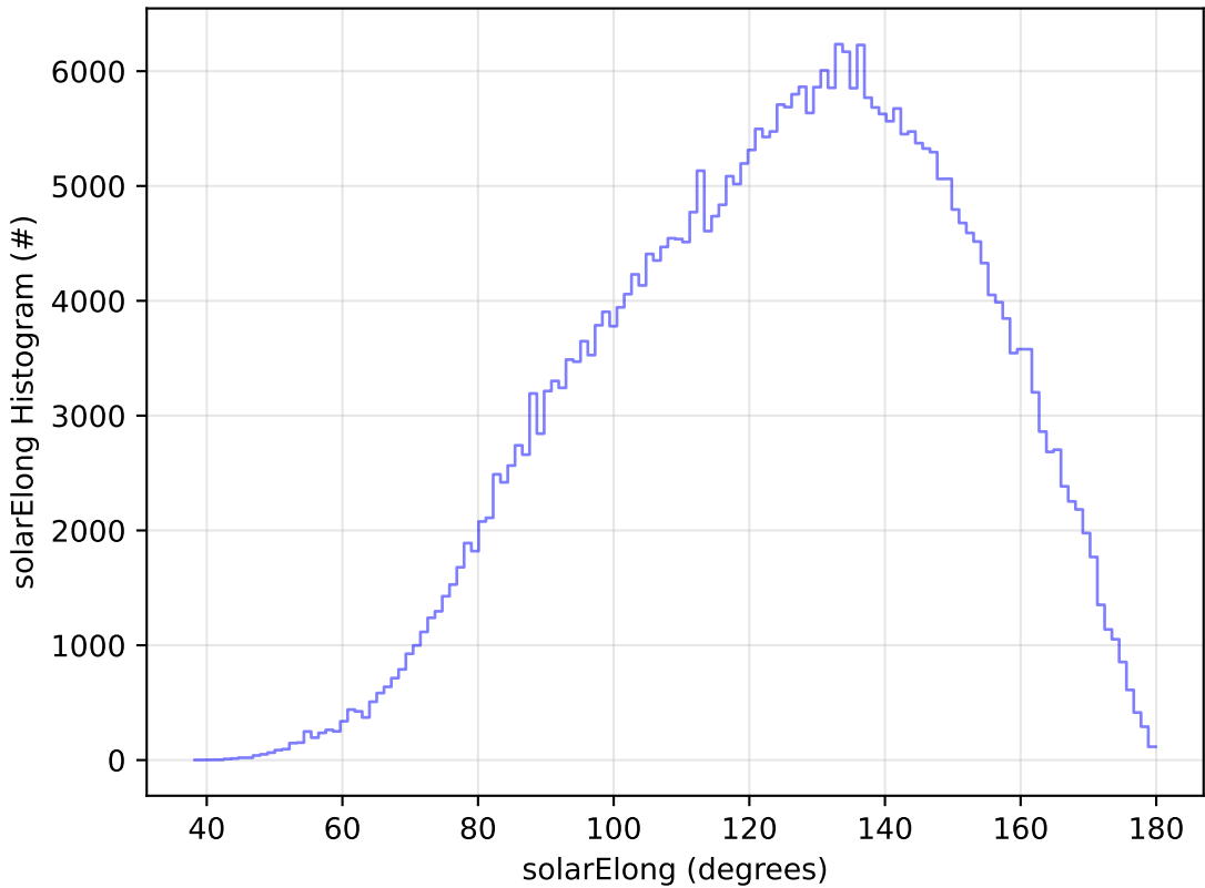
ddf_acor_sf15_lsf40_lsr20_v3.4_10yrs All sky y band: solarElong Histogram
