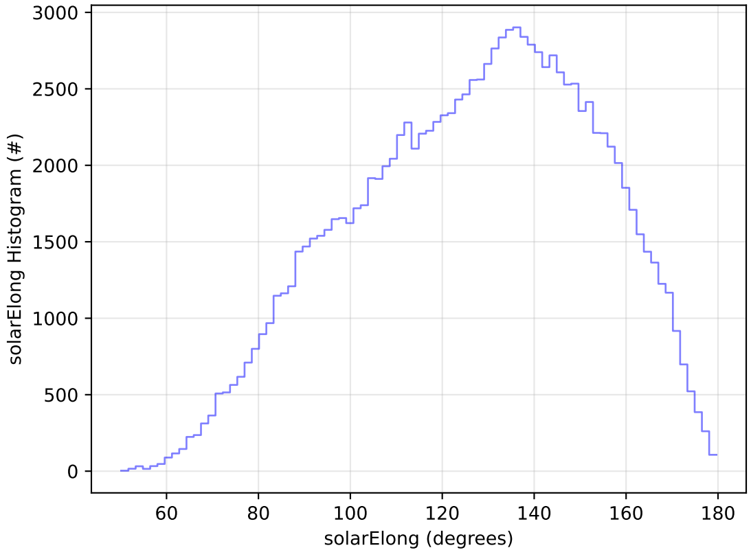
ddf_acor_sf15_lsf40_lsr20_v3.4_10yrs All sky u band: solarElong Histogram
