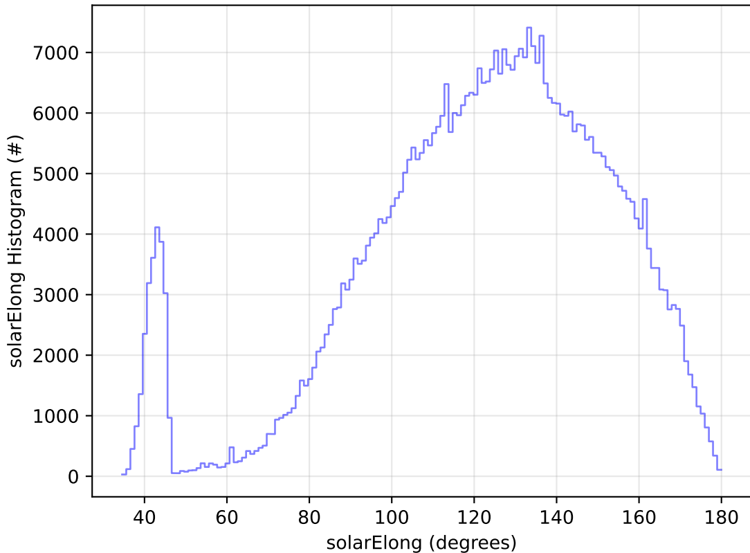
ddf_acor_sf15_lsf40_lsr20_v3.4_10yrs All sky i band: solarElong Histogram
