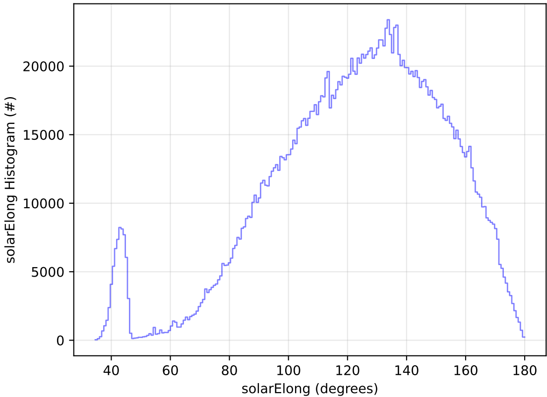
ddf_acor_sf15_lsf40_lsr20_v3.4_10yrs All sky all bands: solarElong Histogram
