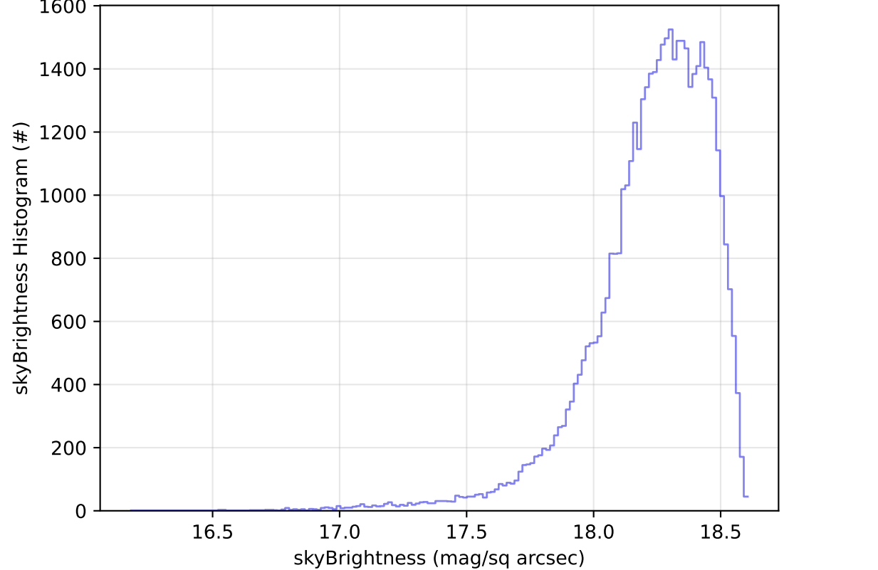
ddf_acor_sf15_lsf40_lsr20_v3.4_10yrs Yr 1 y band: skyBrightness Histogram
