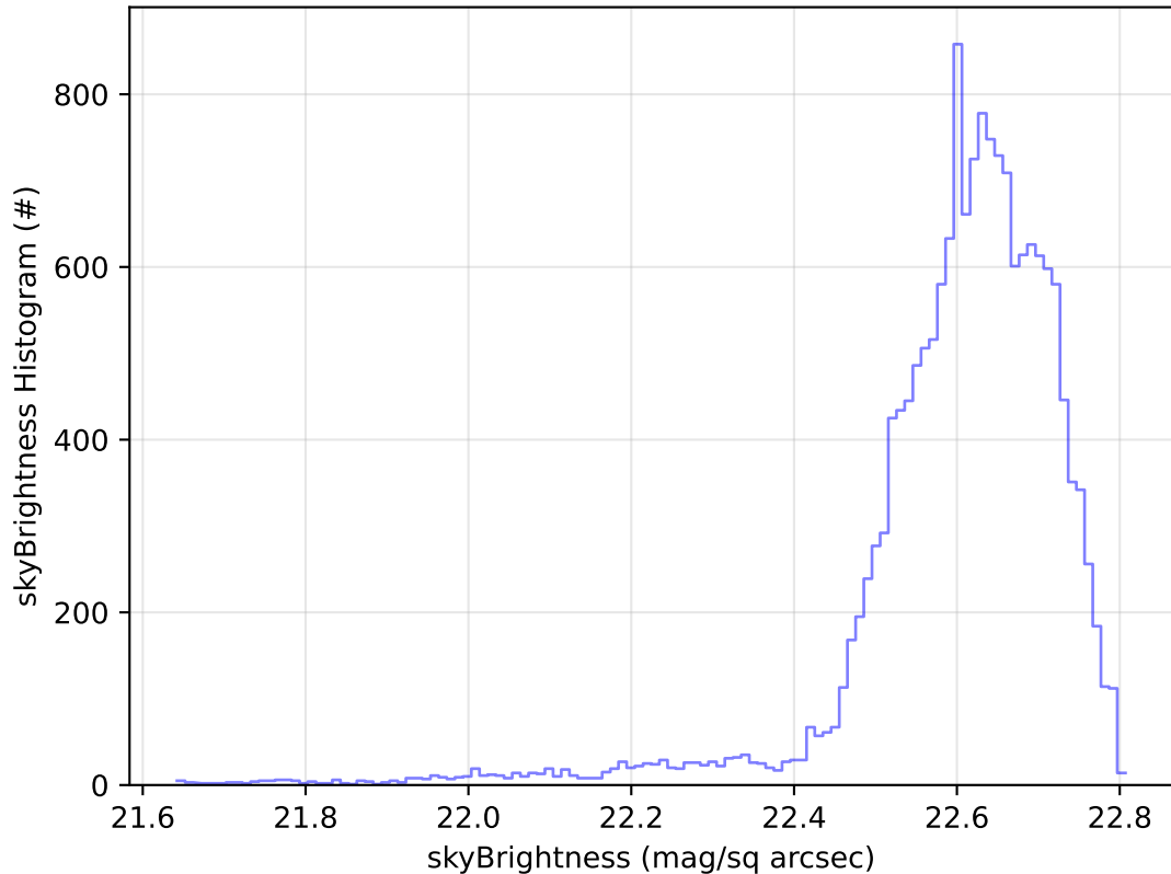
ddf_acor_sf15_lsf40_lsr20_v3.4_10yrs Yr 1 u band: skyBrightness Histogram
