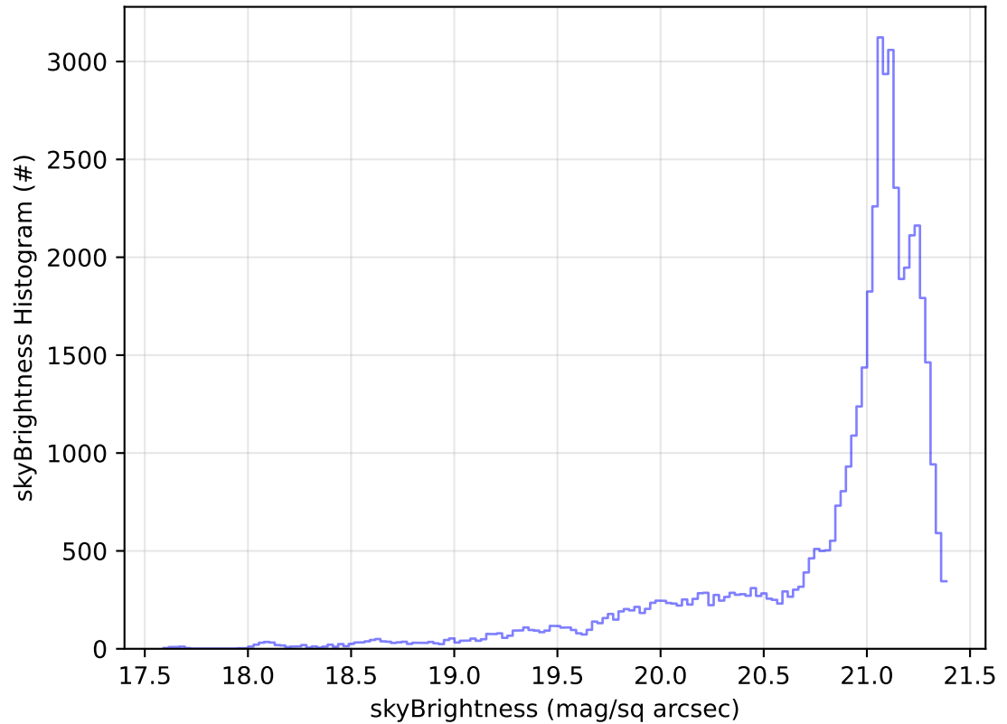
ddf_acor_sf15_lsf40_lsr20_v3.4_10yrs Yr 1 r band: skyBrightness Histogram
