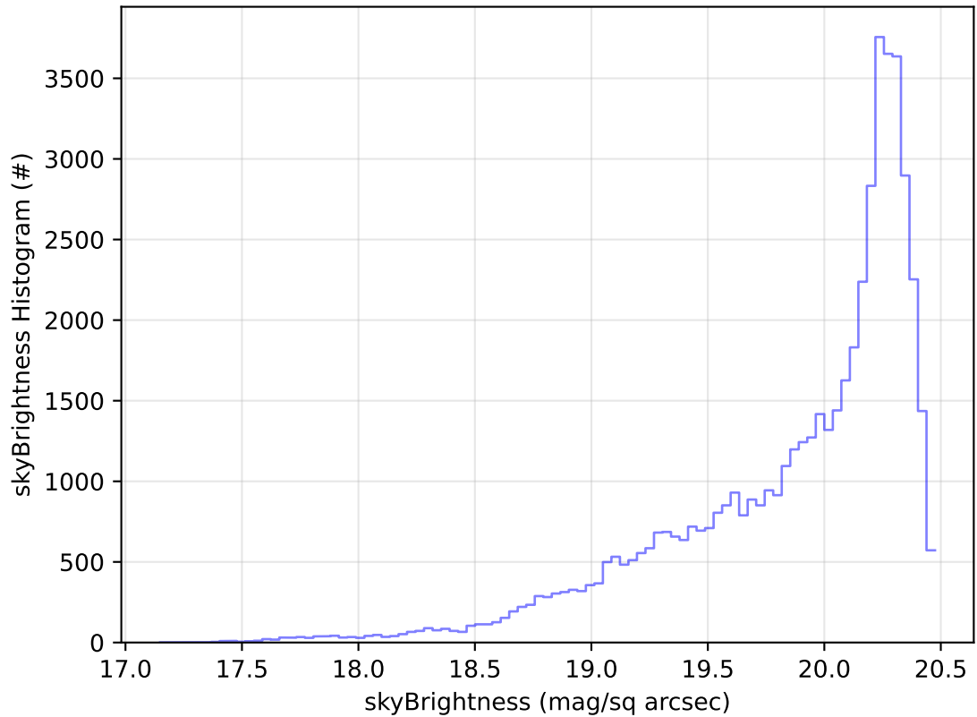
ddf_acor_sf15_lsf40_lsr20_v3.4_10yrs Yr 1 i band: skyBrightness Histogram
