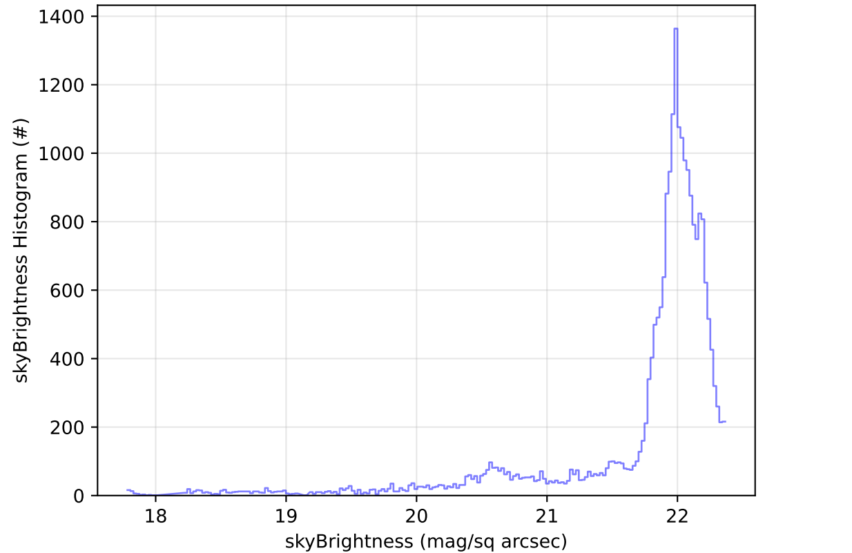
ddf_acor_sf15_lsf40_lsr20_v3.4_10yrs Yr 1 g band: skyBrightness Histogram
