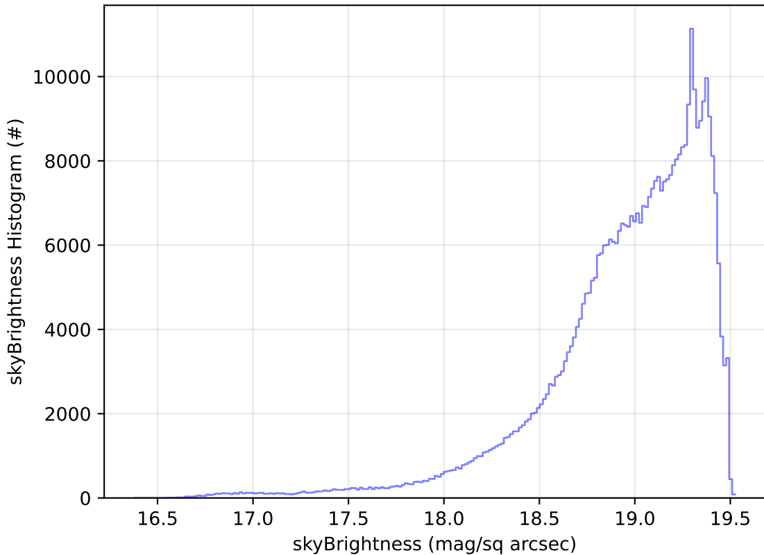
ddf_acor_sf15_lsf40_lsr20_v3.4_10yrs WFD z band: skyBrightness Histogram
